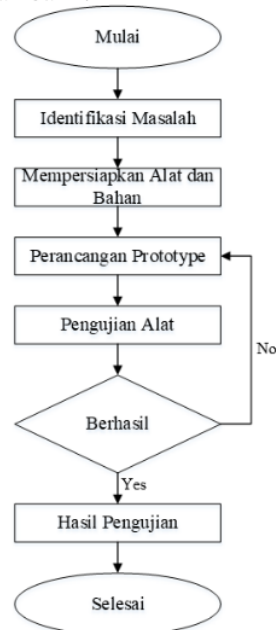
Gambar 1 Flowchart Penelitian
